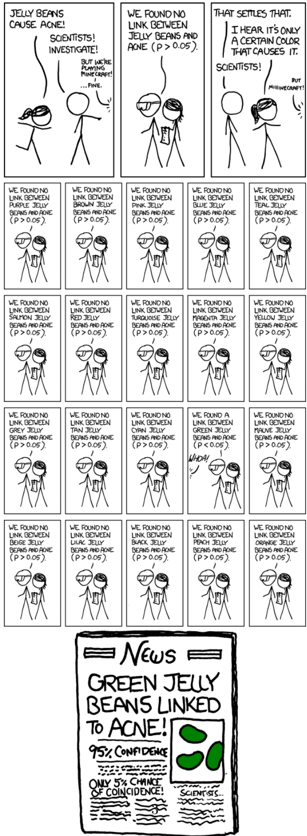
Figure 2: Significant http://xkcd.com/882/
